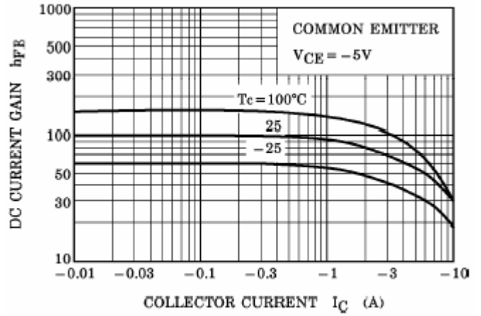
Fig.4 DC current Gain
