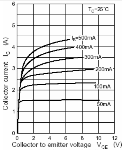
Fig.3 Static Characteristic
